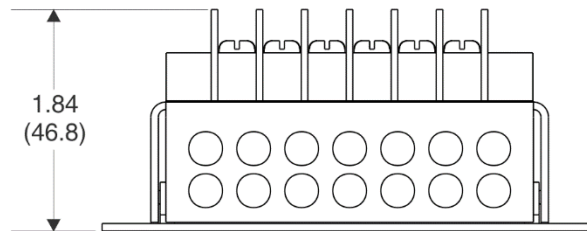
Figure 1. ICRM Dimensions
